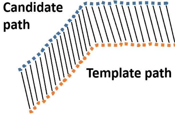
Figure 5.9: Template matching algorithm finding the Euclidean distance between each point on the candidate path (scan-path) to a corresponding point on the template path.
