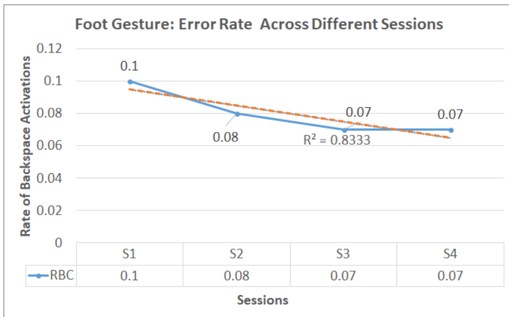
Figure 4.16: Foot gesture-based Selection: error rate expressed in terms of Rate of Backspace Activation (RBA) across different sessions. We observe that the error rate decreases with subsequent sessions, and the regression line has an R^2 value of 0.83
