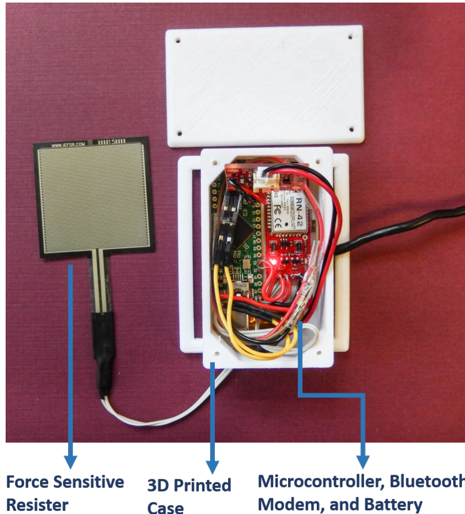
Figure 4.11: Foot Press Sensing Device: the entire circuitry is housed inside a 3D-printed container, and the force sensitive resister that senses foot press actions extends from the main circuit and is placed inside the footwear.
